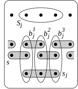
Fig. 1. Reduction from the proof of Lemma 2
