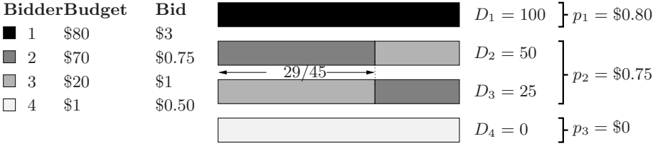
Fig. 2. Consider the same bidders and slots as in Figure 1, but now add bids as shown. Running Find-Price-Block on only bidder 1 gives a price of r_1 = 80/100 , which is less than the next bid of $1. So, we run Find-Price-Block on bidders 1 and 3 (the next-highest bid), giving r_1 = 80/100 and r_2 = 100/150 . We still get a price of $0.80, but now this is more than the next-highest bid of $0.75, so we allocate the first bidder to the first slot at a price of $0.80. We are left with bidders 2-4 and slots 2-4. With just bidder 3 (the highest bidder) and slot 2, we get a price p = 20/50 which is less than the next-highest bid of $0.75, so we consider bidders 2 and 3 on slots 2 and 3. This gives a price of \max\{70/50, 90/75\} = \$1.40 , which is more than $0.50. Since this is also more than $0.75, we must lower B_2 until the price is exactly $0.75, which makes B'_2 = \$36.25 . With this setting of B'_2 , Find-Price-Block allocates bidders 2 and 3 to slots 2 and 3, giving 75(36.25/56.25) and 75(20/56.25) clicks respectively, at a price of $0.75 per click. Bidder 4 is allocated to slot 4, receiving zero clicks.
