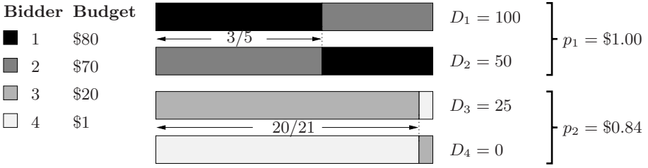
Fig. 1. An example of the PS mechanism (multiple slots, budgets only). The first application of Find-Price-Block computes r_1 = B_1/D_1 = 80/100 , r_2 = (B_1 + B_2)/(D_1 + D_2) = 150/150 , r_3 = (B_1 + B_2 + B_3)/(D_1 + D_2 + D_3) = 170/175 , r_4 = (B_1 + B_2 + B_3 + B_4)/(D_1 + D_2 + D_3 + D_4) = 171/175 . Since r_2 is largest, the top two slots make up the first price block with a price p_1 = r_2 = \$1 ; bidder 1 gets 80 clicks and bidder 2 gets 70 clicks, using the schedule as shown. In the second price block, we get B_3/D_3 = 20/25 and (B_3 + B_4)/(D_3 + D_4) = 21/25 . Thus p_2 is set to 21/25 = \$0.84 , bidder 3 gets 500/21 clicks and bidder 4 gets 25/21 clicks, using the schedule as shown.
