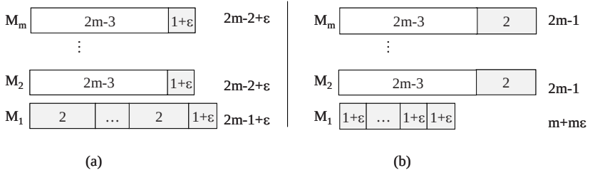
Fig. 4. An LPT-based coalition on m machines in which the job of load 1 + \varepsilon assigned to M_1 has improvement ratio arbitrarily close to 2 - \frac{1}{m}
