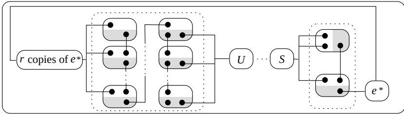
Fig. 3. Gadgets for the proof of Theorem 9. Agents are depicted as rectangles. Shaded areas indicate supplied products, lines connect products of identical type. Again, every feasible non-empty trade must contain agents corresponding to at least r non-intersecting sets.
